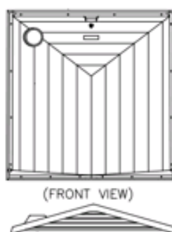
TUFWAY PEAK EASTERN ROOF 1988 TO PRESENT #13298 DRAWING
