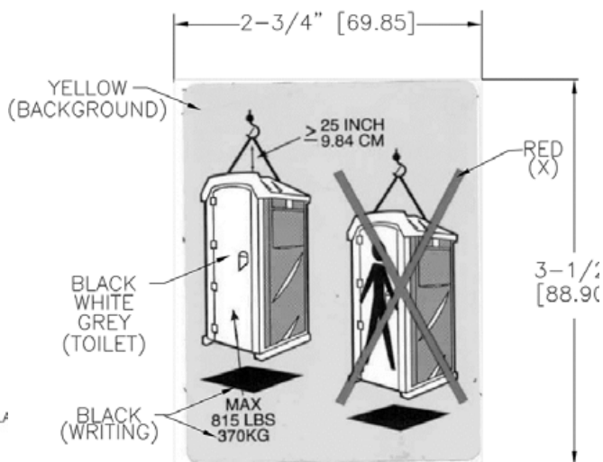
15049 DECAL MX2 WET LIFT
