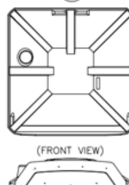
MAXIM 2000 ROOF 1994 TO PRESENT #16167 DRAWING
